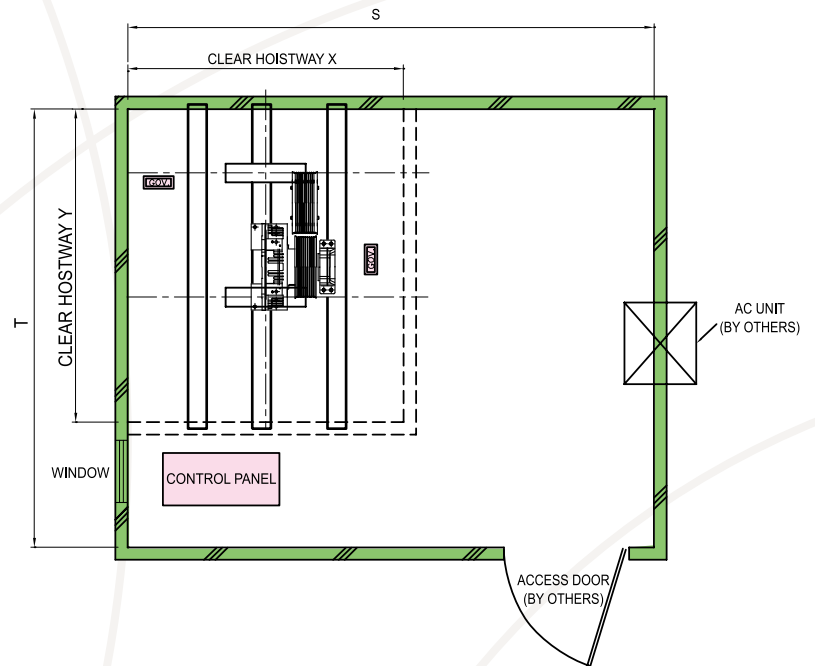
HOISTWAY PLAN
