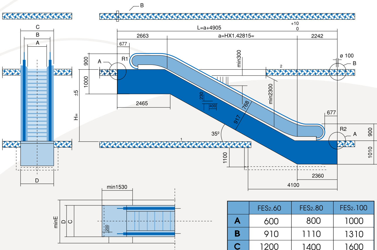
Model FES 30/35
