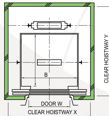
HOISTWAY PLAN
