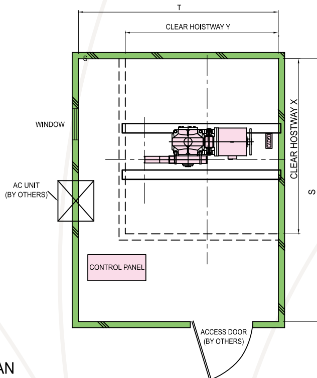
MACHINE ROOM PLAN
