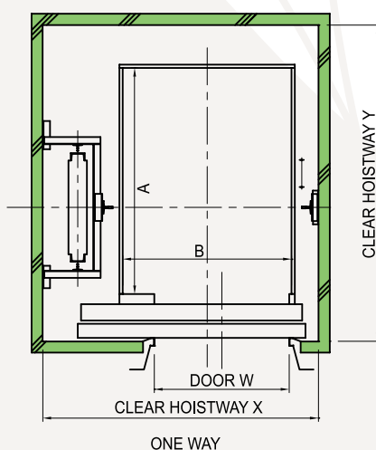
HOISTWAY PLAN
