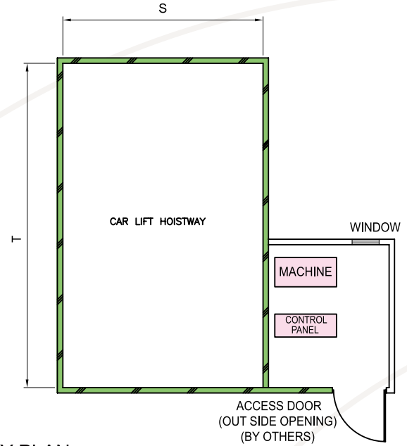
HOISTWAY PLAN
