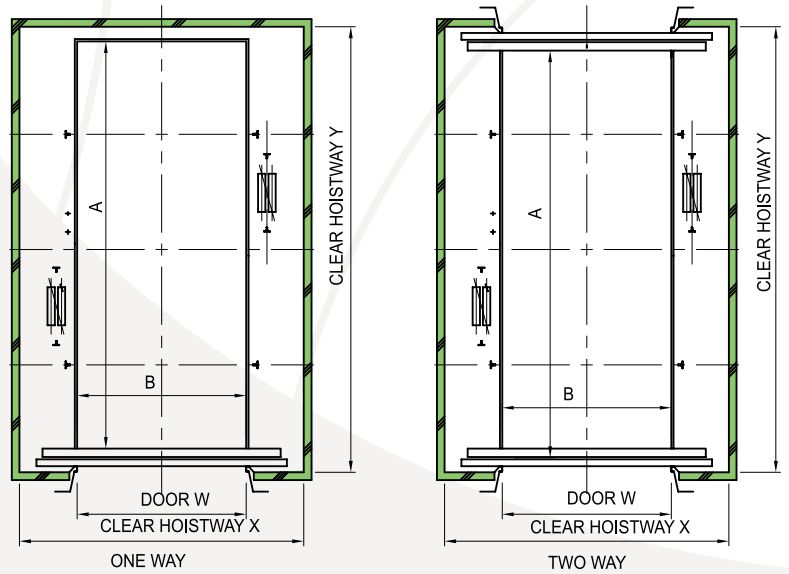
HOISTWAY PLAN
