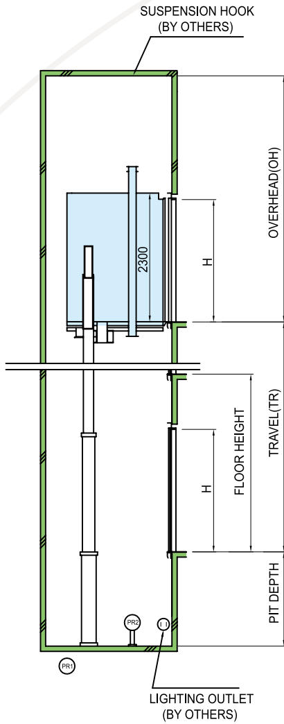
SECTION OF HOISTWAY
